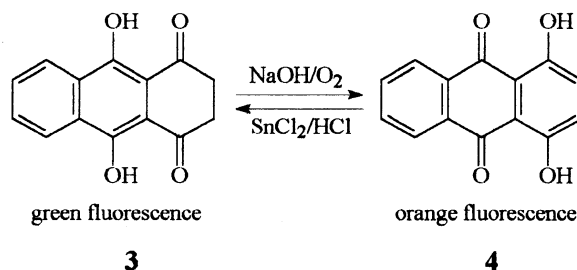
Fig. 4. Oxidation of 2,3-dihydroquinizarin ( 3 ) to quinizarine ( 4 ) by air in the presence of alkali.
