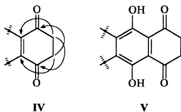
Fig. 3. Substructures IV and V of parimycin constructed from 2D NMR data.
