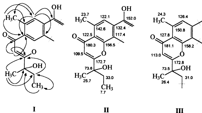
Fig. 2. Substructure I constructed from HMBC ( \rightarrow ) and H,H COSY ( \leftrightarrow ) couplings and developed to II by comparison of the NMR data with those of \gamma - and \delta -indomycinone partial structure III.
