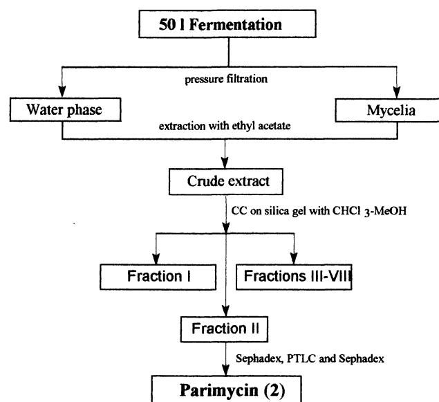
Fig. 1. Working up scheme of the strain Streptomyces sp. isolate B8652.
